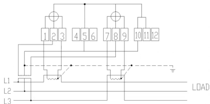
3P3W Asymmetric Connection with CTPT
