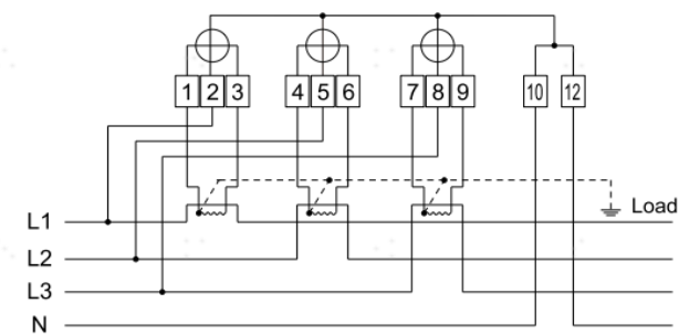
3P4W Asymmetric Connection with CTPT
