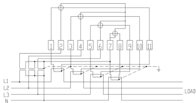
3P4W symmetric Connection with CT
